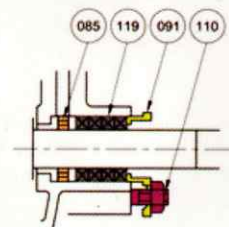
Gland Packing with Lantern Ring
