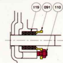
Gland Packing without Lantern Ring
